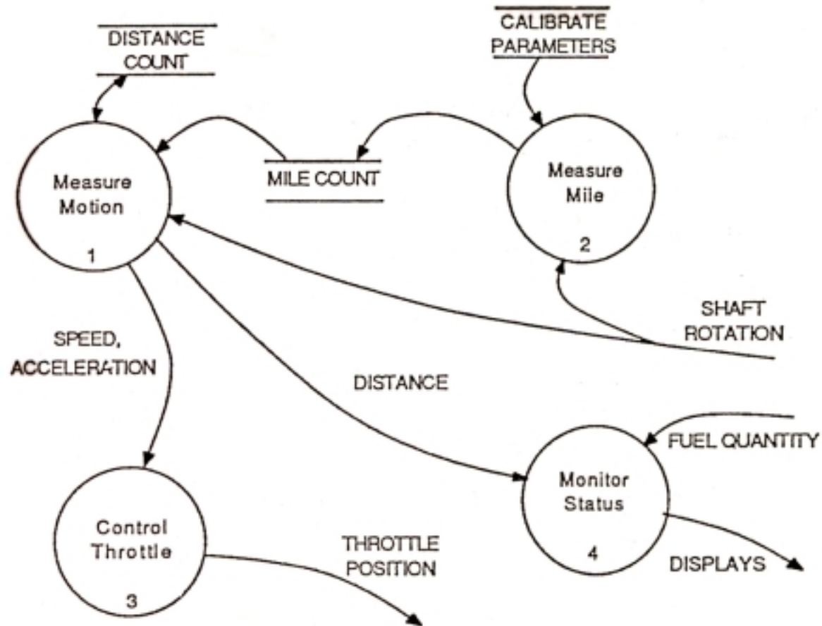
DFD 0; Control & Monitor Auto
