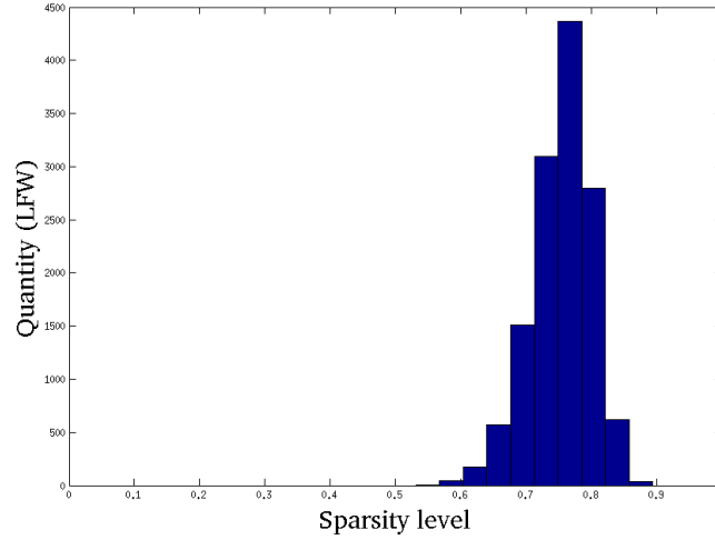
Figure 6. Histogram of the face representation sparsity level on LFW
