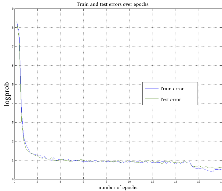
Figure 7. Train and Test errors observed during training on the SFC , over epochs
